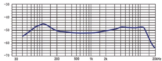
Frequency Response Curve
